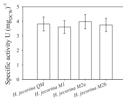
Fig. 4. Specific extracellular \beta -galactosidase activity of H. jecorina QM9414 and GAL10^{1068-2100} -expressing strains M1, M2a, and M2b. Samples were taken 12 h after the transferring procedure.
